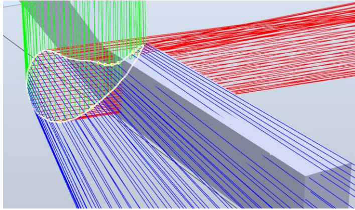
Fig. 3.19. Programmed masticatory trajectory path in the RobotStudio software
