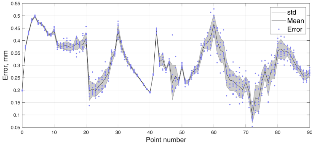
Fig. 4.2. RMSE of every measured point in 10 iterations of cubic test trajectory with mean and standard deviation
