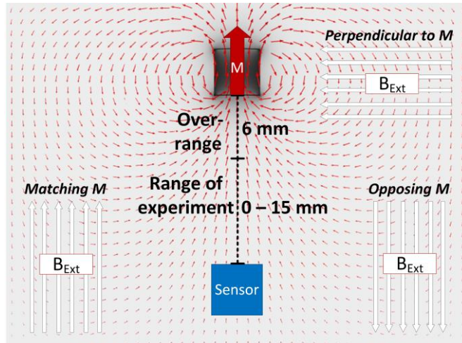
Fig. 3.6. Principle of evaluating the influence of BMF vector B_{EXT} acting in various directions
