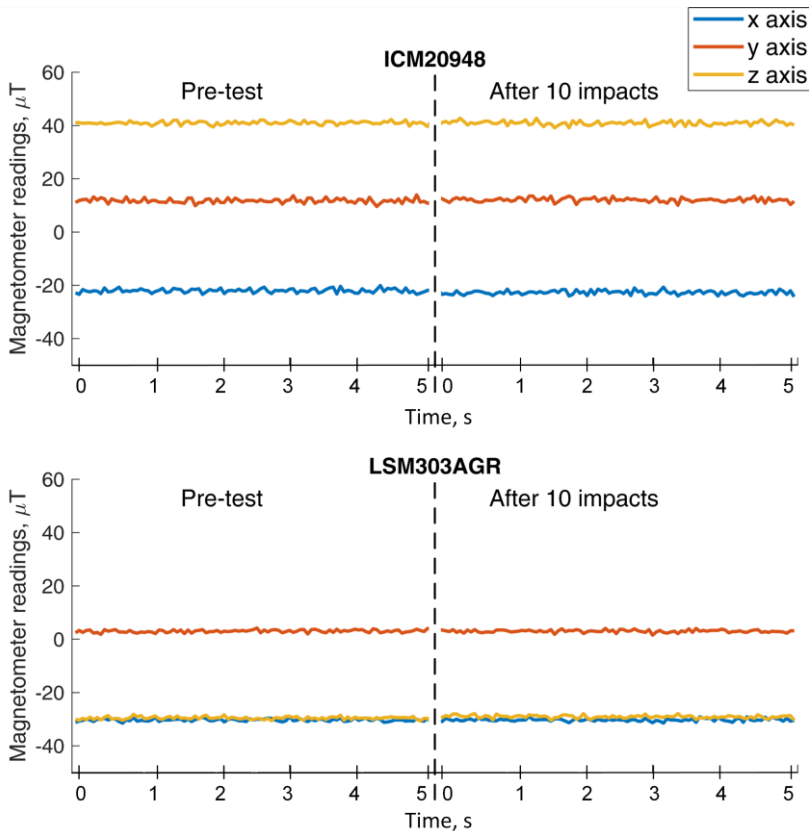
Fig. 4.18. Comparison of ICM20948 and LSM303AGR; zero-offsets not affected by the mechanical shock
