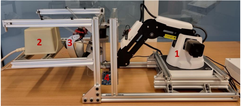
Fig. 3.20. Robot-controlled articulator platform
