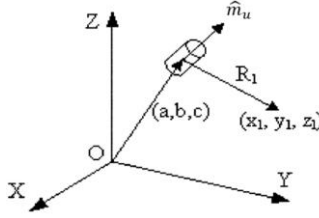
Fig. 2.3. Variables describing a magnetic dipole in a coordinate system [45]
