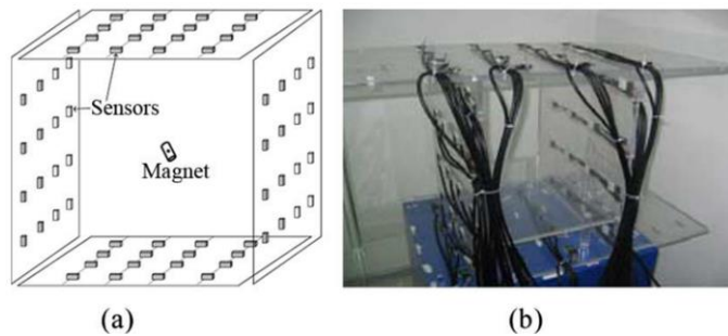
Fig. 2.1. Cubic magnetic sensor array, (a) cubic magnetic sensor array scheme, (b) real cubic magnetic sensor array [52]
